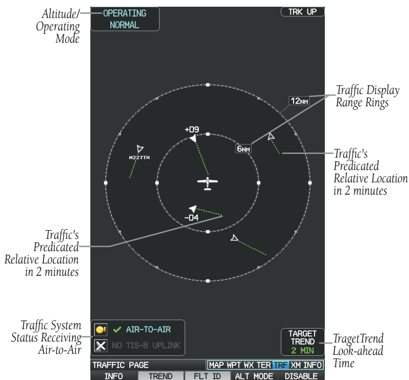
Traffic Page TargetTrend (GDL 39)
