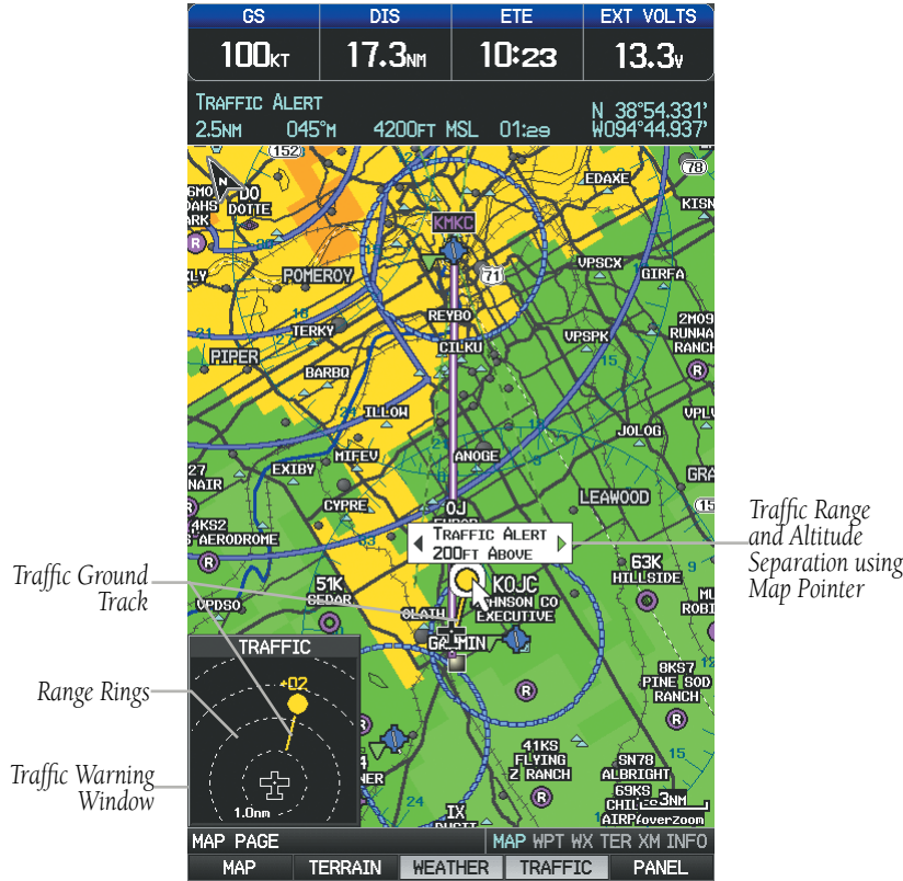
TIS-A (Map Page)
